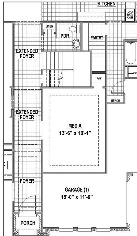
Stair Location with Optional 2nd Floor
