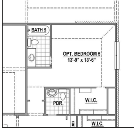
Optional Bedroom 5 with Bath
